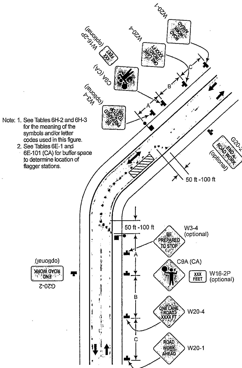
Typical Application 10
